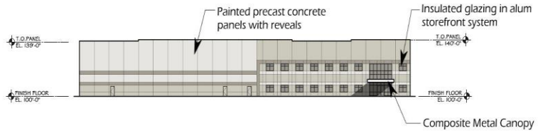
SOUTH ELEVATION
