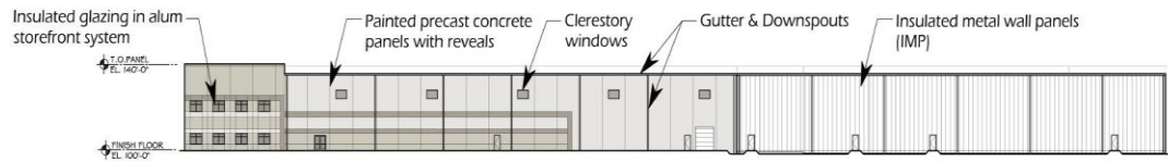
EAST ELEVATION
