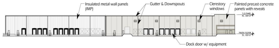
WEST ELEVATION
