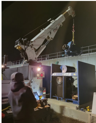
Removing Blower Motor at WWTP
